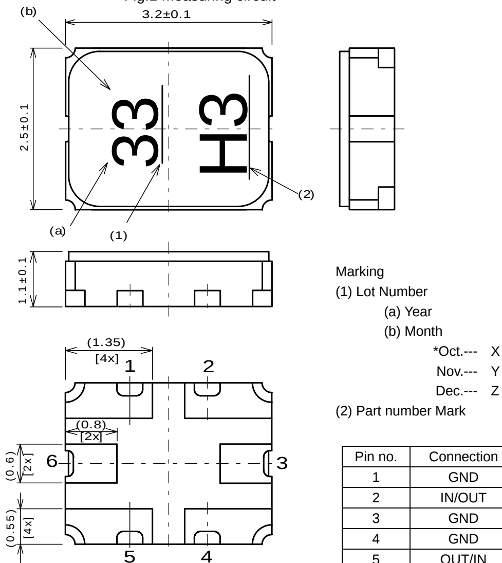
Fig.2 Package dimensions (in mm)
